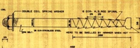
DETAIL OF RAG BOLT
