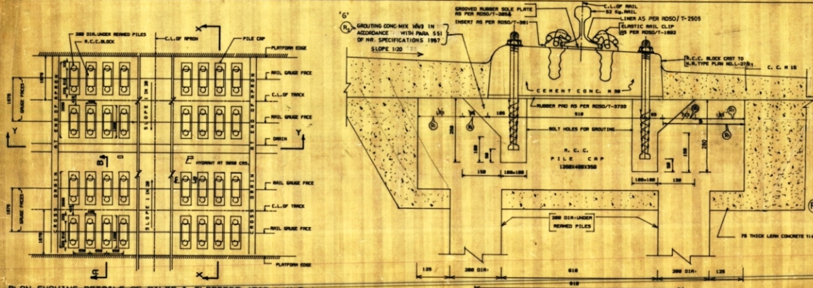
PLAN SHOWING DETAILS OF PILES &amp; SLEEPERS (FOR L.V.R.)
