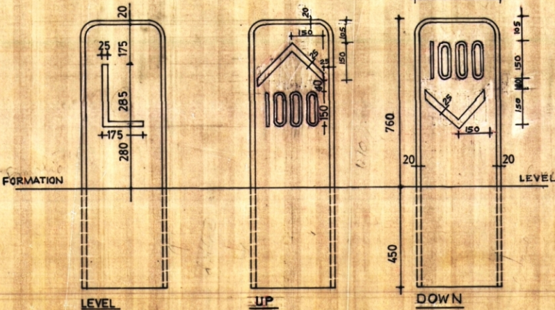
ELEVATIONS (SCALE 1:10)
