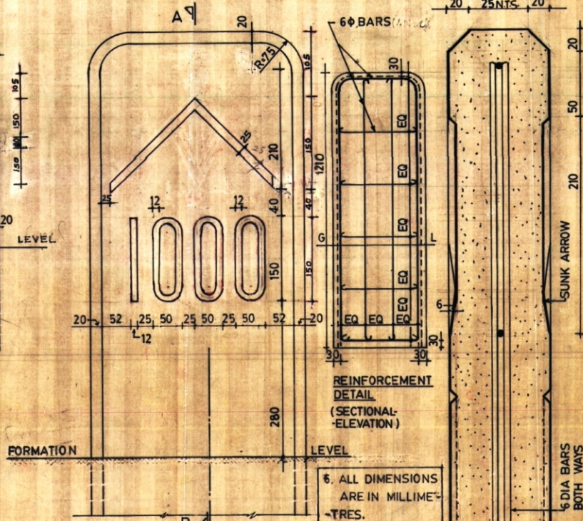
ELEVATION (PART-DETAILED)
