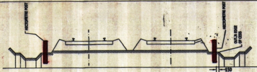
TYPICAL SECTION (THROUGH CUTTING)
