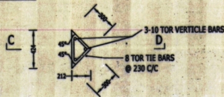
DETAILED PLAN OF HECTOMETRE-POST
