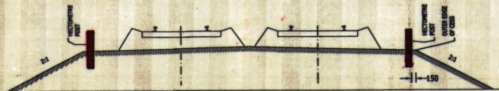
SECTION A-B (THROUGH FILLING)
