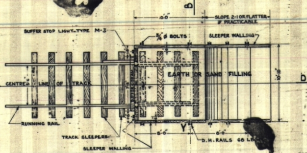
DETAIL AT Y FIXING OF SLEEPERS WITH RAIL UPRIGHTS
