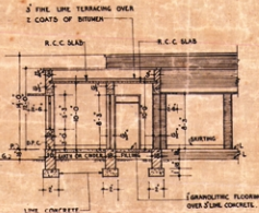
SECTION ON BB
