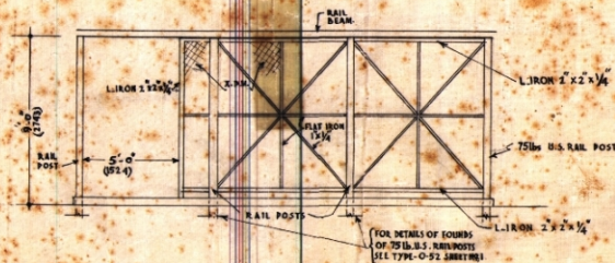
L-SIDE ELEVATION
