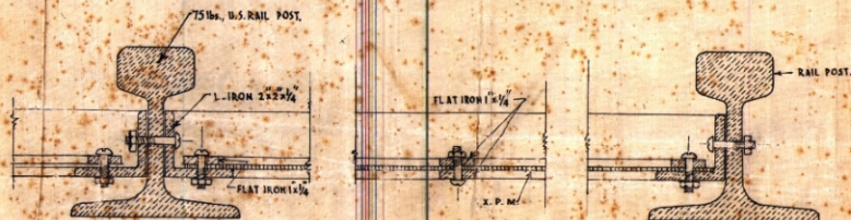
DETAIL OF 'A' SCALE :- HALF FULL SIZE
