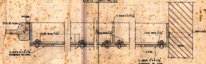
DETAIL OF 'B' SCALE:— HALF FULL SIZE
