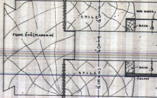
FULL SIZE DETAIL OF WINDOWS FRAME & STILES FOR DOUBLE SHUTTERS
