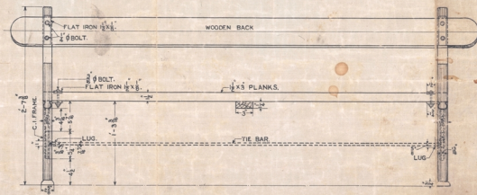
—CROSS SECTION OF C.I.FRAME ON C.D.—
