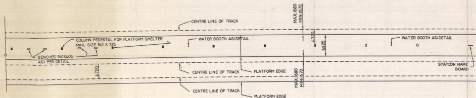
PLAN OF ISLAND PLATFORM EXTENSION WITH RESTRICTED WIDTH
