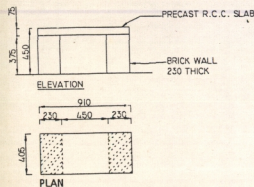
DETAIL OF BENCH
