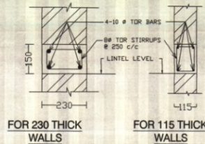
TYPICAL LINTEL BEAM
